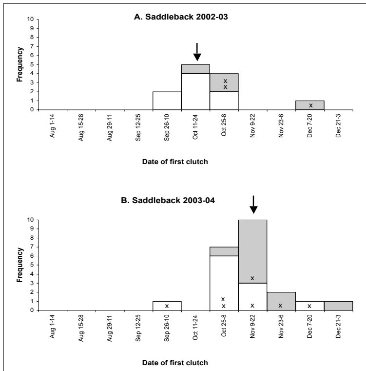
Figure 2 Frequency histogram of dates of first clutches for experienced (open bars) and inexperienced (grey bars) breeding pairs of South Island saddlebacks on Ulva Island in 2002-03 (A) and 2003-04 (B). Arrow indicates overall median date of first clutches and 'x' within bars indicates the number of pairs that were handled.
