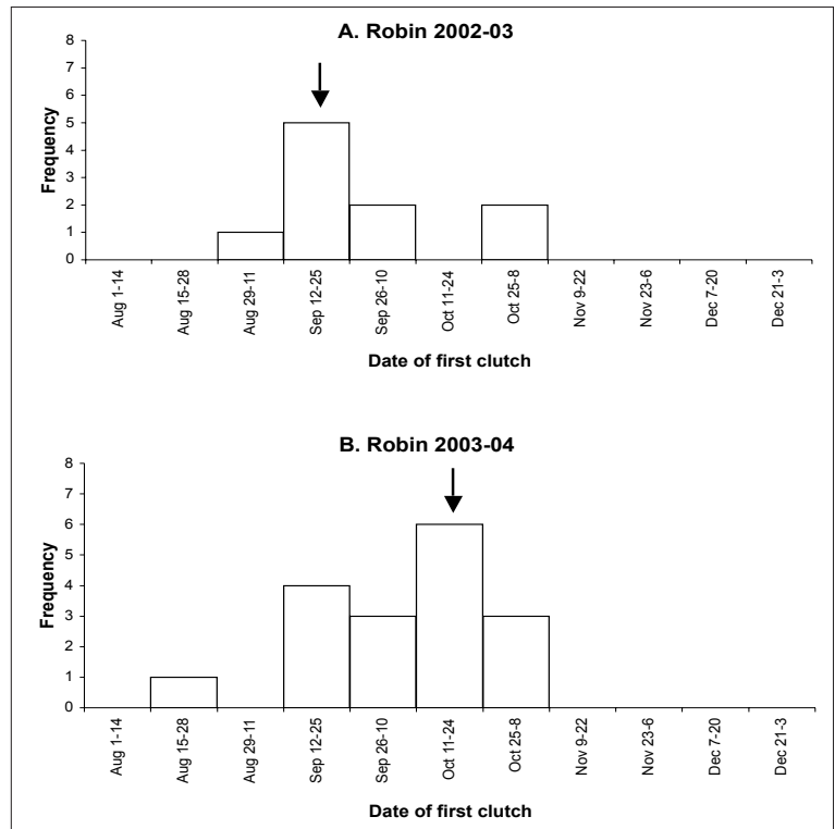
Figure 3 Frequency histogram of dates of first clutches for breeding pairs of Stewart Island robins on Ulva Island in 2002-03 (A) and 2003-04 (B). Arrow indicates median date of first clutches.
