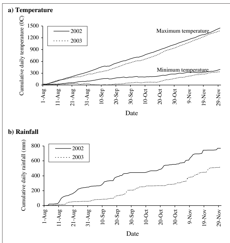
Figure 5 Comparison of the cumulative daily minimum/maximum temperatures and rainfall between 2002 and 2003, for the period from 1 August to 30 November (i.e. leading up to and during the egg-laying period of South Island saddlebacks and Stewart Island robins).
