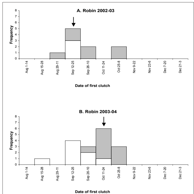
Figure 4 Frequency histogram of dates of first clutches for experienced (open bars) and inexperienced (grey bars) breeding pairs of Stewart Island robins on Ulva Island in 2002-03 (A) and 2003-04 (B). Arrow indicates overall median date of first clutches.
