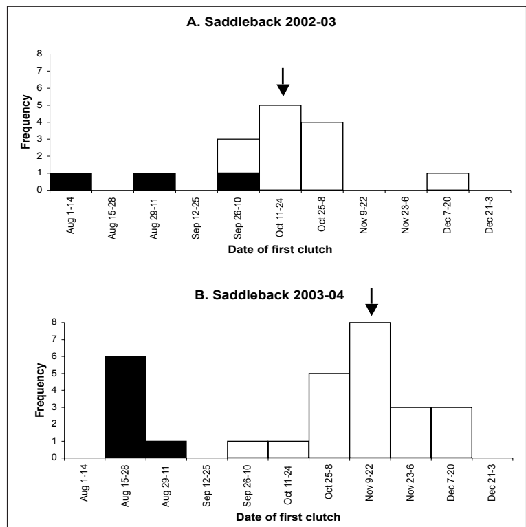
Figure 1 Frequency histogram of dates of capture (black bars) and dates of first clutches (open bars) for breeding pairs of South Island saddlebacks on Ulva Island in 2002-03 (A) and 2003-04 (B). Arrow indicates median date of first clutches.
