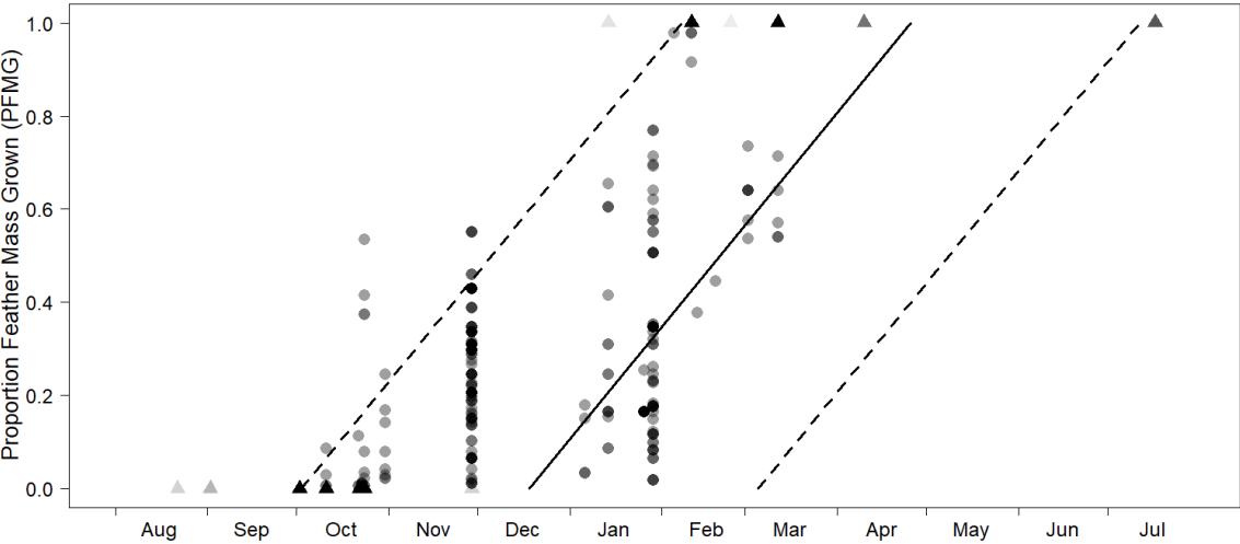
Figure 2. Modified scatter diagram of PFMG for second-year wrybills ( Anarhynchus frontalis ). The straight line links the estimated start date with the estimated end date using PFMG as the moult index and data type 3 of the Underhill-Zucchini moult model. It shows the progression of primary moult for the average second-year bird in the population. The dashed lines are the 95% intervals derived from the standard deviation of the mean start date and the parallelogram enclosed by them should contain 95% of second-year birds in active moult. The circle data points are the birds in active primary moult which were used to estimate the parameters of the moult model. The triangle data points are pre- and post-moult birds that were not used in the model. Intensity of shading from light to dark represents the number of overlapping records at each point: for both circles and triangles the lightest shade represents one data point; the darkest circles represent 7 overlapping data points, while the darkest triangles represent 181 overlapping data points.
